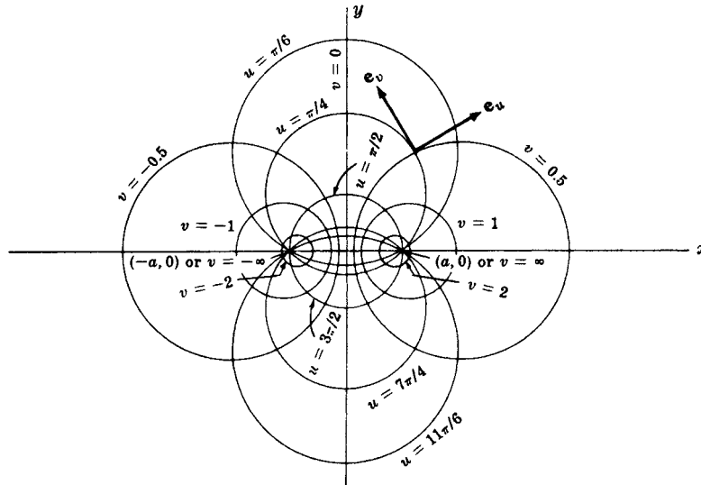
Fig. 20-16. Bipolar coordinates.
