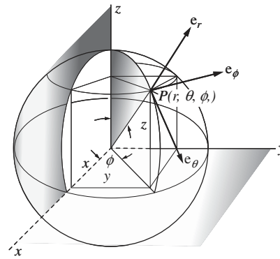
Fig. 20-13. Spherical coordinates.
