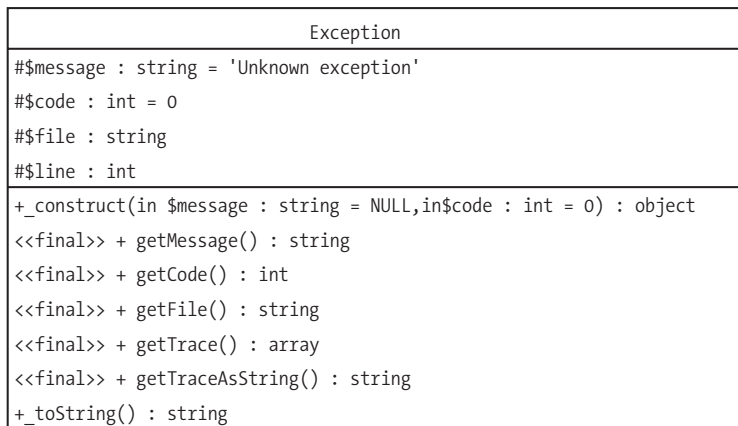
Figure 2-5. The PHP 5 Exception class (UML representation)
